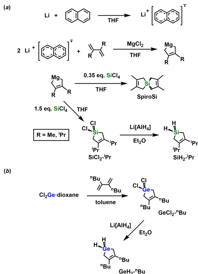
Scheme 1 (a) Synthesis of silaspiro-[4.4]-2,3,7,8-tetramethyl-2,7-nona-1,5-diene (SpiroSi) and 1,1-dihydro-3,4-di-iso-propylsilacyclopent-3-ene ( \text{SiH}_2-\text{iPr} ); (b) synthesis of 1,1-dichloro-3,4-dibutylgermacyclopent-3-ene \text{GeCl}_2-\text{nBu} and 1,1-dihydro-3,4-dibutylgermacyclopent-3-ene \text{GeH}_2-\text{nBu} .
