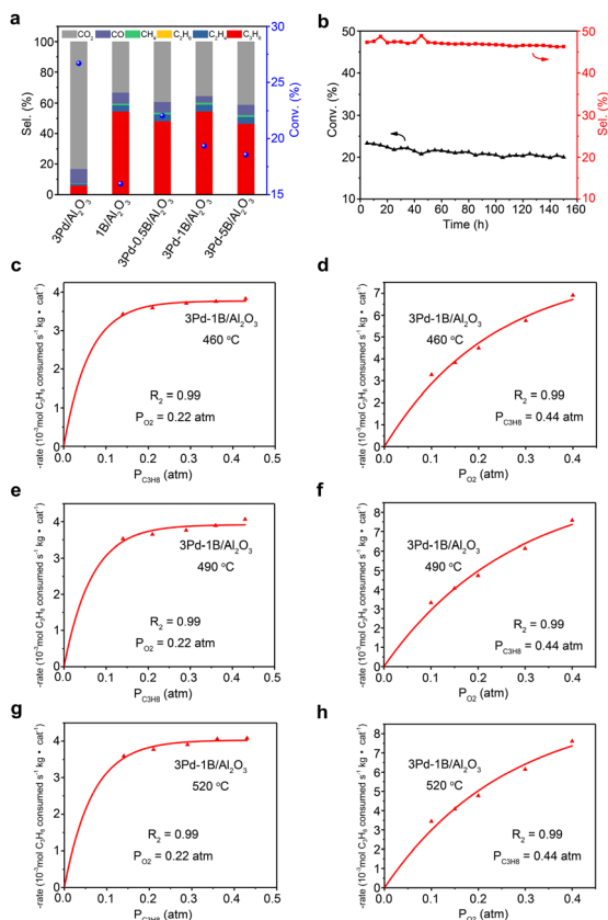
Fig. 1 (a) Catalytic performance of ODHP over 3Pd/Al 2 O 3 , 1B/Al 2 O 3 and 3Pd-1B/Al 2 O 3 catalysts after 1 hour. (b) Propane conversion and propylene selectivity over time on stream for 3Pd-1B/Al 2 O 3 . Conditions: 490 °C, WHSV -1 = 0.29 g C 3 H 8 -1 g catalyst hours, WHSV = 1800 L C 3 H 8 kg catalyst -1 h -1 , P C 3 H 8 :P O 2 :P N 2 = 4.4:2.2:93.4 kPa. (c) Rates of propane consumption using 3Pd-1B/Al 2 O 3 as a function of P C 3 H 8 (P O 2 constant at 0.22 atm) at 460 °C. (d) Rates of propane consumption using 3Pd-1B/Al 2 O 3 as a function of P O 2 (P C 3 H 8 constant at 0.44 atm) at 460 °C. (e and f) Corresponding propane consumption rates at 490 °C. (g and h) Corresponding propane consumption rates at 520 °C.
