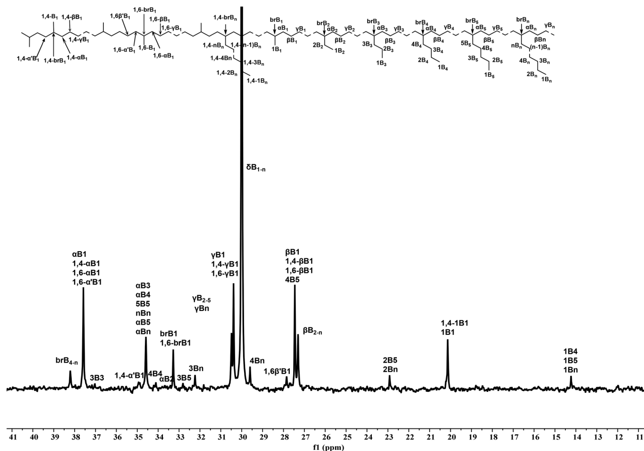
Fig. 2 ^{13}\text{C} NMR spectrum of PE-Ni1 produced using Ni1/EASC (run 7, Table 2) in the region \delta 11–41 ppm; recorded in \text{C}_2\text{D}_2\text{Cl}_4 at 100 °C.
