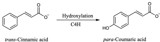
Scheme 1 Hydroxylation of trans -cinnamic acid to para -coumaric acid catalyzed by the P450 enzyme C4H.
