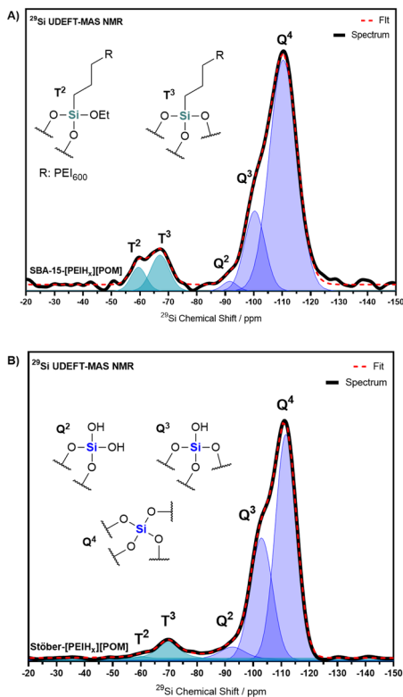
Fig. 3 ^{29}\text{Si} UDEFT NMR spectra of a) SBA-15-[PEI _x ][POM] (A) and Stöber-[PEI _x ][POM] (B), with inset of structures of Si species observed ( T^n : carbon-bonded silicon atoms, Q^n : silanols and siloxanes).
