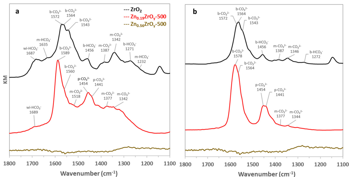
Fig. 6 DRIFT spectra of (a) \text{CO}_2 adsorption at 325 °C and 10 bar on \text{ZrO}_2 , \text{Zn}_{0.19}\text{ZrO}_y -500, and \text{Zn}_{0.56}\text{ZrO}_y -500 after 40 minutes under 2 ml min -1 \text{CO}_2 and 16 ml min -1 Ar and (b) after 40 minutes evacuation at 325 °C and 10 bar under 16 ml min -1 Ar (m: monodentate, b: bidentate, wi: weakly interacting, and p: polydentate species).
