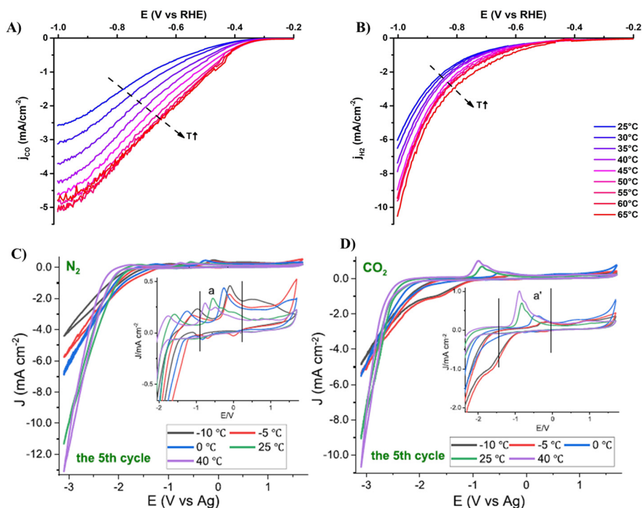
Fig. 18 Partial current density towards CO formation (A) and \text{H}_2 (B) at different temperatures in 0.1 M \text{NaHCO}_3 on a gold RRDE at 2500 rpm and 20 \text{ mV s}^{-1} . 205 Curves (the fifth cycle) of Pt in \text{N}_2 (C) and \text{CO}_2 -saturated, a ( -2 to 2 V), (D) ionic liquid in the potential range of -3.1 to 1.7 V vs. Ag/AgCl, a' ( -2.5 to 2 V). Reproduced with permission. 206 ©2020, the American Chemical Society.
