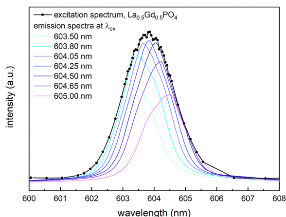
Fig. 6 Luminescence line narrowing can be observed following direct excitation of \text{Cm}^{\text{III}} in solid phases lacking long-range order ( e.g. , amorphous materials), or in systems with random cation distribution, such as disordered (statistical) solid solutions. \lambda_{\text{ex}} refers to excitation wavelength used for the collection of the emission spectra (colored traces). Adapted in part from ref. 51. Copyright 2018 American Chemical Society.
