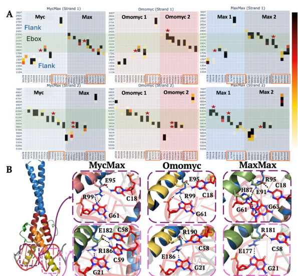
Fig. 5 Protein–DNA hydrogen bond (HB) interactions and patterns in the MycMax, Omomyc dimer, and MaxMax complexes. (A) Heatmaps of HB occupancy for MycMax, Omomyc, and MaxMax complexes interacting with the DNA from individual 1- \mu s MD simulations. HB contacts with the DNA bases are marked with red stars. The E-box region is highlighted in green, and each protein monomer is delimited by a rectangular colored box. The HLH region is delimited by an orange box on the x-axis. (B) Molecular visualization of key protein–DNA HBs. Each monomer is shown in a separate row. The top row shows Myc, Omo1 and Max1, respectively. The bottom row shows Max, Omo2, and Max2, respectively.
