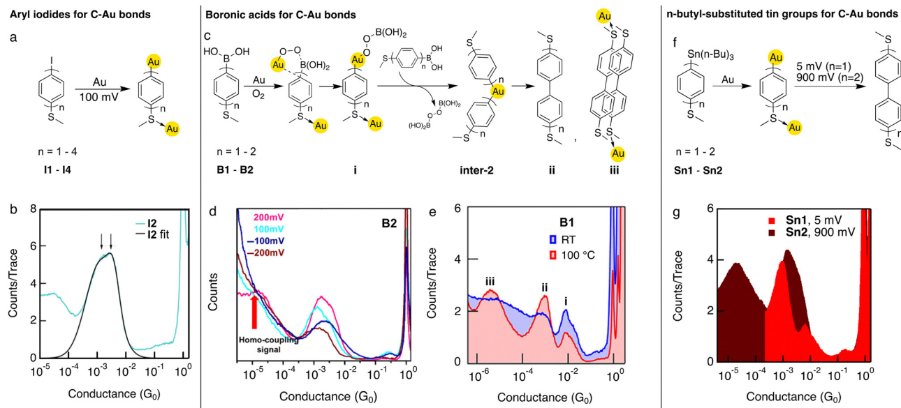
Fig. 3 (a) Schematic illustration of in situ cleavage of aryl iodides in forming junctions with C–Au covalent linkage on one side and a S→Au dative bond on the other. (b) 1D histogram of 12 measured under 100 mV in TCB. The black line represents a double Gaussian fit to the data. (c) Proposed mechanism of in situ cleavage of the organoboron group, homocoupling reaction, and proposed molecular junction for the ultra-low conductance peak labeled as iii . (d) 1D conductance histograms of B2 measured under bias voltages of 200 mV, 100 mV, –100 mV, and –200 mV. (e) 1D conductance histograms of B1 measured in bis(2-ethylhexyl) adipate solvent under room temperature and 100 °C. (f) Schematic illustration of in situ cleavage of the organotin group and homocoupling reaction. (g) 1D conductance histograms of Sn1 and Sn2 measured in TCB under 5 mV and 900 mV bias voltages. (b) is adapted with permission from ref. 52, copyright (2020) American Chemical Society. (d) is adapted with permission from ref. 53, copyright (2022) Chinese Chemical Society. (e) is adapted with permission from ref. 54, copyright (2024) American Chemical Society. (g) is adapted with permission from ref. 57, copyright (2024) American Chemical Society.
