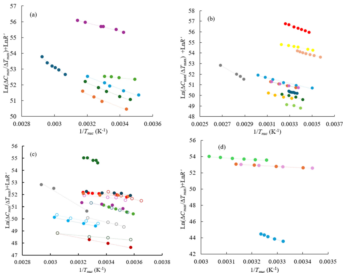
Fig. 2 Plot of \ln(\Delta C_{\max}/\Delta T_{\max}) + \ln R' versus 1/T_{\text{nuc}} for (a) 6 different combinations of API and solvents involving 4 APIs, (b) 11 different combinations of API and solvents involving 6 APIs, (c) combination of inorganics/solvents involving 8 different compounds and (d) API intermediate, amino acid and a large molecule. Note: these values are valid only at the cooling rates studied given in Table 1. Fig. 2a: ●: paracetamol/water ( R' : 0.5 K s -1 ); ●: dextrose/water ( R' : 0.0278 K s -1 ); ●: L-asparagine monohydrate/water ( R' : 0.005 K s -1 ); ●: L-asparagine monohydrate/water ( R' : 0.0033 K s -1 ). Fig. 2b: ●: ibuprofen/ethanol ( R' : 0.0167 K s -1 ); ●: paracetamol/ethanol ( R' : 0.0167 K s -1 ); ●: pyrazinamide/acetone ( R' : 0.0167 K s -1 ); ●: fenofibrate/ethyl acetate ( R' : 0.05 K s -1 ); ●: gestodene/ethanol ( R' : 0.0083 K s -1 ); ●: gestodene/ethanol ( R' : 0.00167 K s -1 ); ●: carbamazepine_saccharine/ethanol ( R' : 0.0167 K s -1 ); ●: pyrazinamide/acetone ( R' : 0.0033 K s -1 ); ●: gestodene/ethanol ( R' : 0.00167 K s -1 ). Fig. 2c: ●: NaNO 3 /NaCl + NaNO 3 + H 2 O solution ( R' : 0.000833 K s -1 ); ●: NaNO 3 /NaCl + NaNO 3 + H 2 O solution ( R' : 0.001667 K s -1 ); ●: CoSO 4 /water ( R' : 0.000833 K s -1 ); ○: CoSO 4 /water ( R' : 0.001667 K s -1 ); ●: CoSO 4 /water ( R' : 0.0025 K s -1 ); ○: (NH 4 ) 2 B 4 O 7 ·4H 2 O/water ( R' : 0.00833 K s -1 ); ○: (NH 4 ) 2 B 4 O 7 ·4H 2 O/water ( R' : 0.0025 K s -1 ); ●: Na 3 VO 4 /NaOH solution ( R' : 0.005 K s -1 ); ●: Sr(OH) 2 ·8H 2 O/water ( R' : 0.001388 K s -1 ); ○: Sr(OH) 2 ·8H 2 O/water ( R' : 0.00277 K s -1 ); ●: ZnL 2 /water ( R' : 0.00138 K s -1 ); ○: ZnL 2 /water ( R' : 0.00275 K s -1 ); ●: borax/water ( R' : 0.003472 K s -1 ); ○: borax/water ( R' : 0.01066 K s -1 ); ●: ammonium oxalate/water ( R' : 0.000833 K s -1 – plotted in secondary axis). Fig. 2d: ●: L-arabinose/water ( R' : 0.0083 K s -1 ); ●: glycine/water ( R' : 0.001667 K s -1 ); ●: glycine/water ( R' : 0.005 K s -1 ); ●: lysozyme/NaCl solution ( R' : 0.002778 K s -1 – we assumed this cooling rate – shown in secondary axis).
