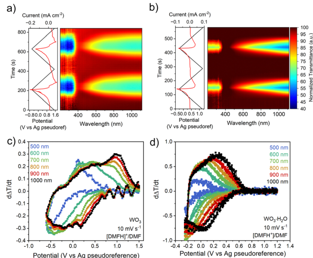
Fig. 4 Operando electrochemical UV-vis-NIR spectra of \text{WO}_3 and \text{WO}_3\cdot\text{H}_2\text{O} collected in 0.1 \text{ M [DMFH]}^+/\text{DMF} and 0.1 \text{ M NBu}_4\text{PF}_6 in MeCN. Color map plots of normalized transmittance as a function of time for \text{WO}_3 (a) and \text{WO}_3\cdot\text{H}_2\text{O} (b) collected at 10 \text{ mV s}^{-1} . Rate of transmittance change, \text{dAT}/\text{dt} , vs. potential for \text{WO}_3 (c) and \text{WO}_3\cdot\text{H}_2\text{O} (d) collected at 10 \text{ mV s}^{-1} .
