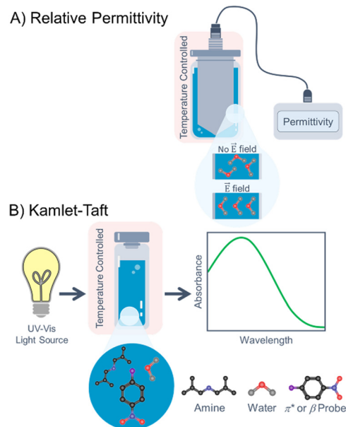
Fig. 1 Schematic illustrating the characterization techniques for (A) the relative permittivity, \epsilon_r , and (B) the Kamlet–Taft polarity parameters, \pi^* and \beta .
