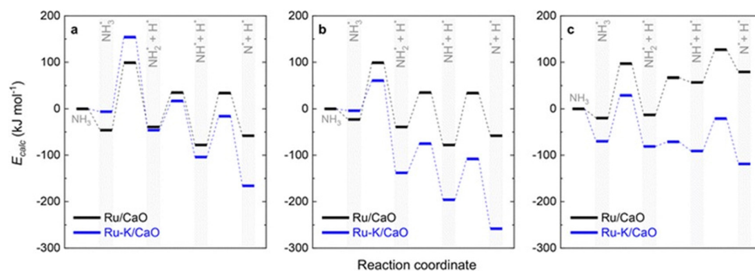
Fig. 20 Potential surface diagrams considering the obtained activation energies from the fitted models: (a) case A (NH 3 dissociation); (b) case B (N 2 desorption); and (c) case C (NH 2 dissociation). (Reproduced with permission from ref. 166 from the Royal Society of Chemistry).
