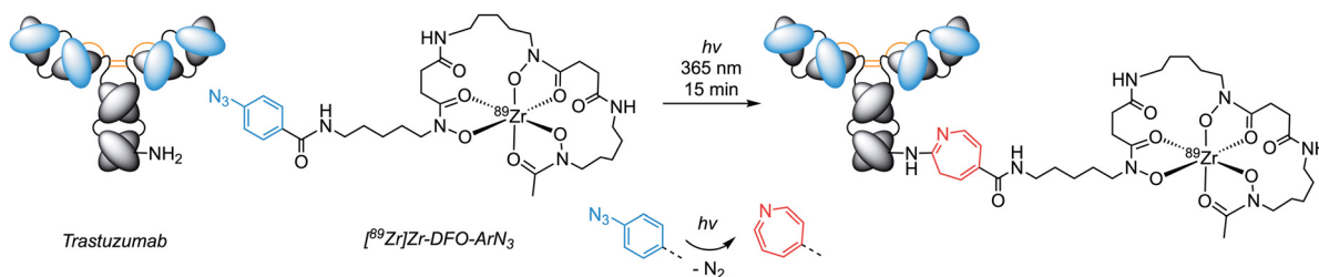
Scheme 3 Photoradiosynthesis to label a monoclonal antibody with a positron-emitting 89 Zr-desferrioxamine complex via light-induced activation of a \text{ArN}_3 group. Trastuzumab is linked in a one-pot photoreaction to [ 89 Zr]ZrDFO- \text{ArN}_3 with high isolated and decay-corrected radiochemical yields and radiochemical purities. 28,53,54
