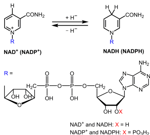
Fig. 1 Structural forms of \text{NAD(P)}^+ and \text{NAD(P)H} .
