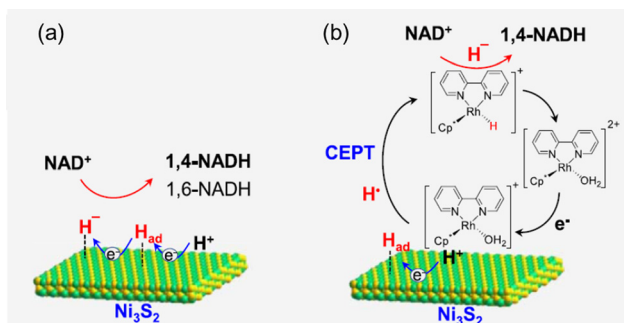
Scheme 8 Proposed mechanisms of \text{NAD}^+ reduction into \text{NADH} for (a) \text{Ni}_3\text{S}_2 alone and (b) the \text{Ni}_3\text{S}_2 -Rh system. Reprinted with permission from ref. 53. Copyright 2024, American Chemical Society.
