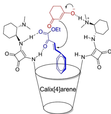
Fig. 8 Control of the distance between two substrates by calix[4]squaramide. Reproduced with permission from ref. 134, copyright 2020 Elsevier Publishing Group.
