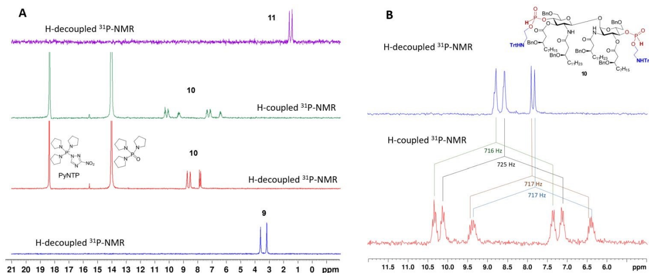
Figure 2. Analysis of the H-phosphonate coupling step by ^{31}\text{P} -NMR. (A) The progress of the H-phosphonate coupling reaction 9 \rightarrow 11 followed by ^{31}\text{P} -NMR; (B) ^{31}\text{P} -NMR spectrum of the H-phosphonate diester 10 prior to oxidation step.
