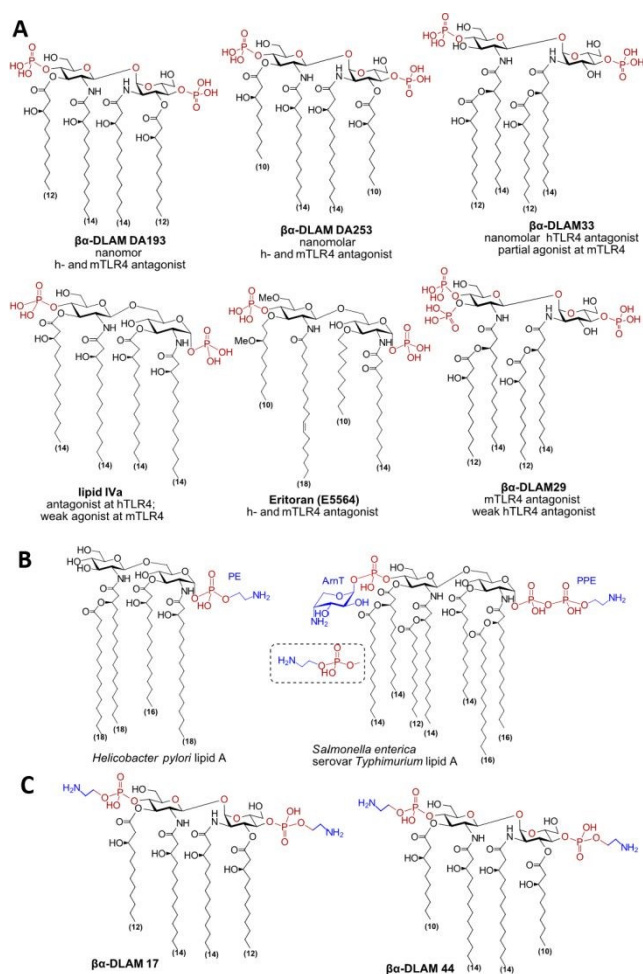
Figure 1. (A) Chemical structure of synthetic TLR4 antagonists; (B) examples of PE-modified lipid A variants; (C) target PE-glycolipids.
