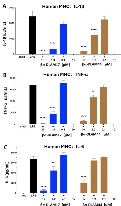
Figure 3. Antagonistic potential of \beta\alpha -DLAM17 and \beta\alpha -DLAM44 in human mononuclear cells (MNC). Inhibition of E.coli O111:B4 LPS [10 ng/mL]-induced release of IL-1 \beta (A), TNF- \alpha (B), and IL-6 (C). Data shown are combined from n=5 independent donors; error bars indicate standard error of the mean.
