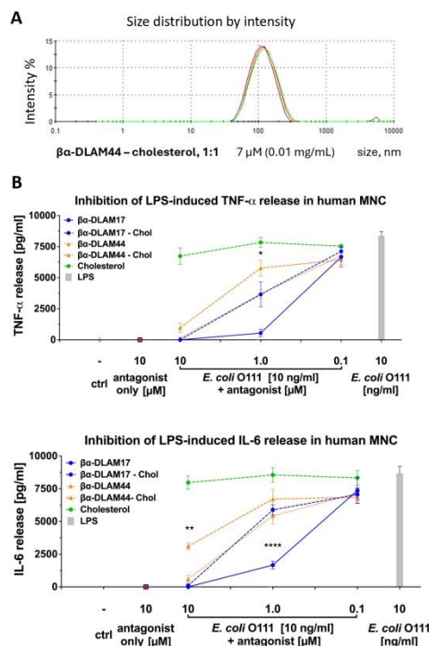
Figure 5. (A) Liposomal formulation of \beta\alpha -DLAM44 analysed by DLS; (B) TLR4-antagonistic potential of PE-modified glycolipids included in cholesterol-containing liposomes. Data shown are combined from n = 5 independent donors; error bars indicate standard error of the mean.
