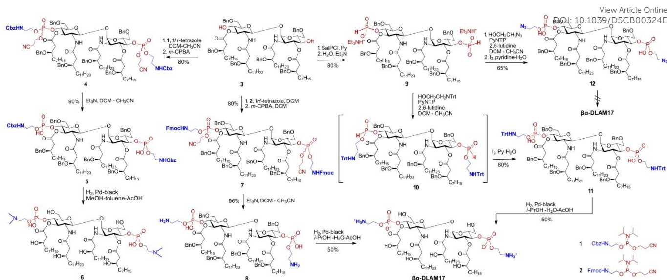
Scheme 1. Synthesis of PE-modified glycolipid \beta\alpha -DLAM17
