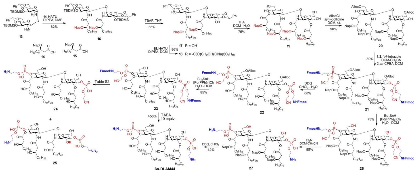
Scheme 2. Synthesis of PE-modified glycolipid \beta -DLAM44
