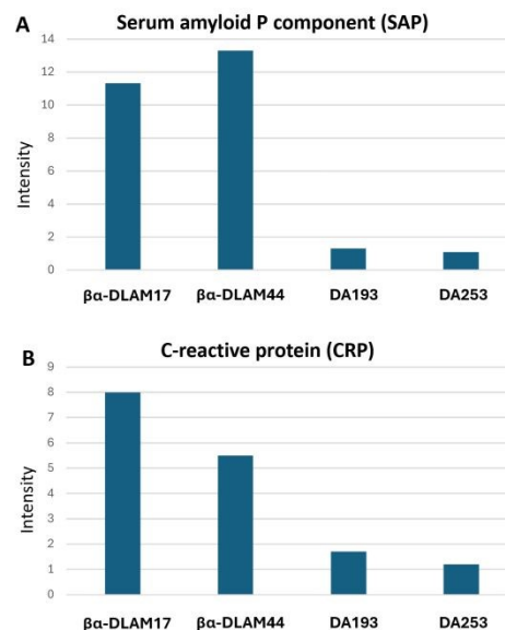
Figure 6. Interaction of \beta\alpha -DLAMs with SAP and CRP by dot blot assay with quantification by densitometry using relative quantification by ImageJ.
