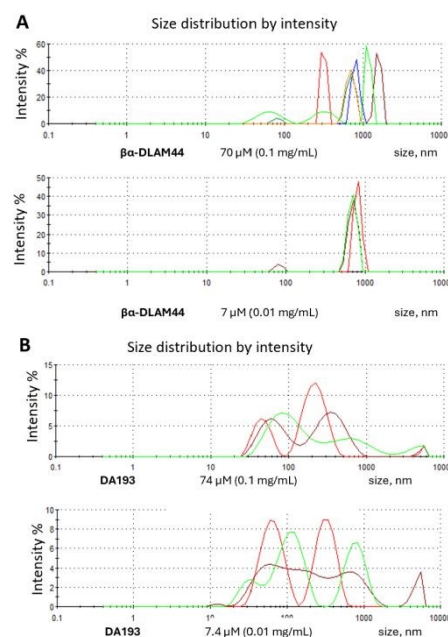
Figure 4. Analysis of aggregation properties of PE-modified \beta\alpha -DLAM44 and unmodified diphosphate DA193 by DLS.
