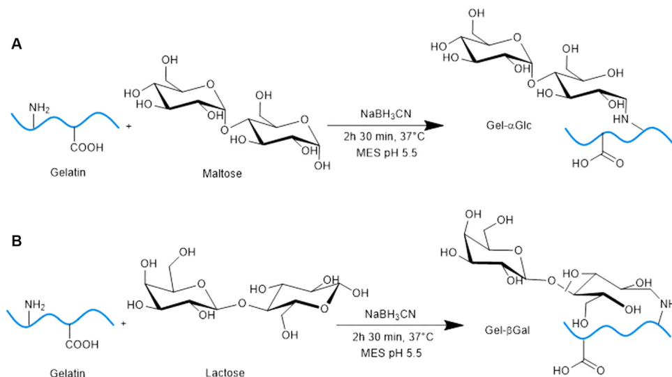
Scheme 1 Functionalization of gelatin with αGlc (A), Gel-αGlc and βGal (B), Gel-βGal by reductive amination with maltose and lactose, respectively exploiting the lysine residues of the protein.
