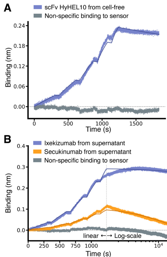
Fig. 4 Characterisation of scFv binding in the pico-molar range. (A) Binding sensorgrams of SpyTagged scFv HyHEL10 (PDB ID 2znrw) loaded from cell-free-expression mixture and binding to purified hen egg-white lysozyme, which was used as analyte at increasing concentrations of 0.31, 0.625, 1.25, 2.5, and 5 nM. The solid lines correspond to a fit with a 1:1 standard binding model (fit RMSE \cong 0.007 nm, \cong 2.7% of the response window). (B) Binding sensorgrams of SpyTagged scFv Ixekizumab and Secukinumab (see legend) loaded from a mammalian-cell supernatant and binding to IL-17A, which was used as analyte at increasing concentrations of 0.25, 0.5, 1, 2, and 4 nM. The association phase is plotted on a linear scale (x-axis), while the much longer dissociation phase on a log 10 scale. The solid lines correspond to a fit with a 1:1 standard binding model (fit RMSE \cong 0.005 nm and 0.004 nm, \cong 1.7% and 3.5% of the response window, respectively for Ixekizumab and Secukinumab).
