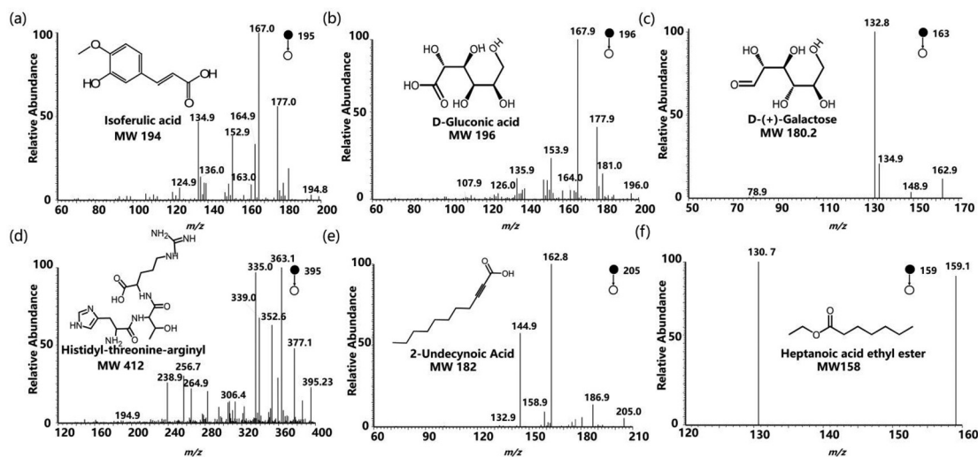
Fig. 5 ND-EESI-MS spectra of differential ions in MiXi beverage treated with different heating conditions: (a) isoferulic acid; (b) D-gluconic acid; (c) D-(+)-galactose; (d) histidinyl-threonine-arginyl; (e) 2-undecynoic acid; (f) heptanoic acid ethyl ester.
