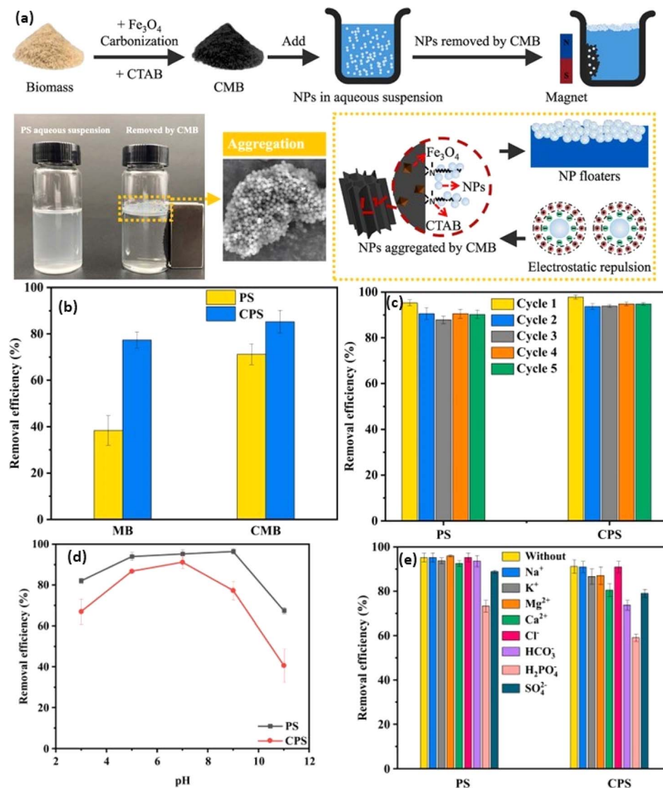
Fig. 4 (a) Synthesis of magnetic biochar (MB) and CTAB modified biochar (CMB), (b) removal efficiency of PS (PS) and carboxylate modified PS (CPS), (c) reusability, (d) pH stability, and (e) highly selective in the presence of a wide variety of metal ions. 136
