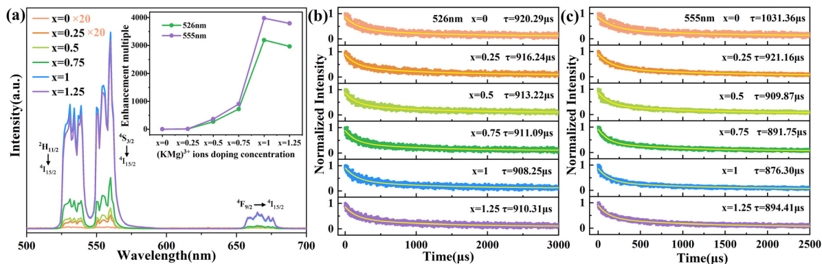
Fig. 5 (a) Upconversion emission spectra of (\text{KMg})_x\text{Sc}_{2-x}\text{W}_3\text{O}_{12}:1 \text{ mol\% Er}^{3+}/20 \text{ mol\% Yb}^{3+} ( x = 0, 0.25, 0.5, 0.75, 1, \text{ and } 1.25 ) phosphors, inset: multiple luminescence enhancement of the phosphor with different (\text{KMg})^{3+} concentrations. Photoluminescence decay curves of \text{Er}^{3+} : (b) {}^2\text{H}_{11/2} and (c) {}^4\text{S}_{3/2} in phosphors monitored at 370 nm.
