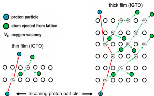
Fig. 25 Schematic diagram of the mechanism for a significant increase in the O_{\text{vac}} concentration in thicker IGTO thin films after proton irradiation based on the multiple displacement chain reaction model. Reproduced with permission. 195 Copyright 2024, Surface and Interfaces.
