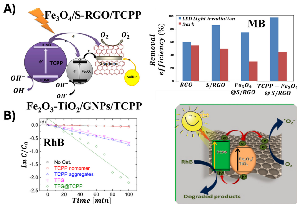
Fig. 33 (A) Mechanism of MB photodegradation catalyzed by \text{Fe}_3\text{O}_4/\text{S-RGO/TCPP} . Adapted with permission from ref. 156. Copyright 2015, Springer Science Business Media Dordrecht. (B) Mechanism of RhB photodegradation catalyzed by \text{Fe}_2\text{O}_3\text{-TiO}_2/\text{GNPs/TCPP} . Adapted with permission from ref. 155. Copyright 2021 Elsevier Ltd.
