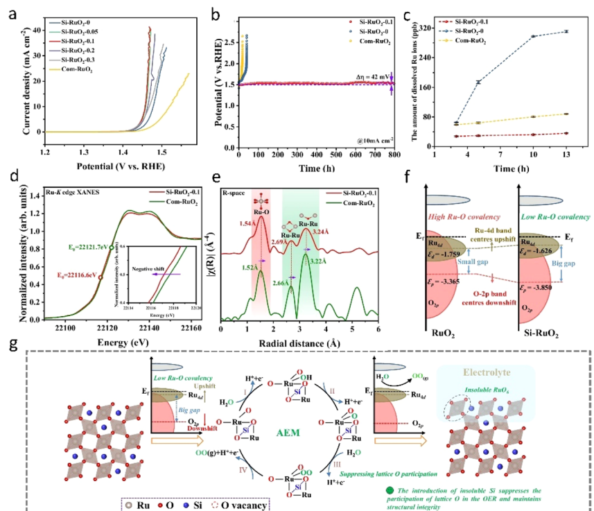
Fig. 10 (a and b) OER performance of the prepared Si-RuO 2 in acidic electrolyte. (c) Comparison of the number of leached Ru ions during the OER process observed for Si-RuO 2-x and com-RuO 2 . (d) Normalized Ru K-edge XANES spectra of Si-RuO 2-0.1 and com-RuO 2 . (e) Fourier-transform EXAFS spectra of Si-RuO 2-0.1 and com-RuO 2 . (f) Schematic diagram of the band structures of Si-RuO 2 and RuO 2 based on Ru and O atoms on the (110) plane. (g) Schematic diagram of the enhanced stability caused by interstitial Si doping. 81 Copyright 2024, Springer Nature.
