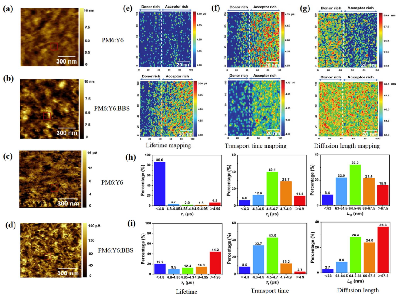
Fig. 4 AFM-topography of (a) PM6:Y6, and (b) PM6:Y6: BBS. c -AFM-conductivity of (c) PM6:Y6 and (d) PM6:Y6: BBS. (e) Carrier lifetime \tau_t , (f) carrier transport time \tau_r , (g) carrier diffusion length L_D . (h and i) Statistical distribution of \tau_t , \tau_r , and L_D for PM6:Y6 and PM6:Y6: BBS organic films. 60 Reproduced from ref. 60 with permission from John Wiley and Sons, copyright 2022.
