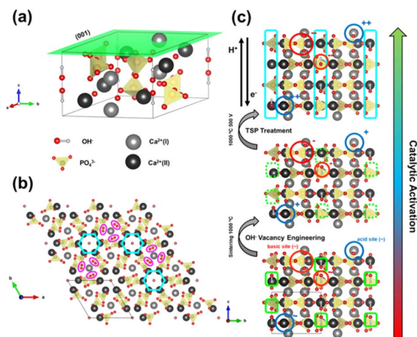
Scheme 1 Structure of HAP as a catalyst. (a) HAP unit cell P6_3/m . (b) (001) crystallographic plane observed from the c -axis direction. The \text{OH}^- channels and the Ca(l) 6-fold coordination are highlighted. (c) Structural changes and lattice refinement strategies adopted to achieve the catalytic activation of HAP.
