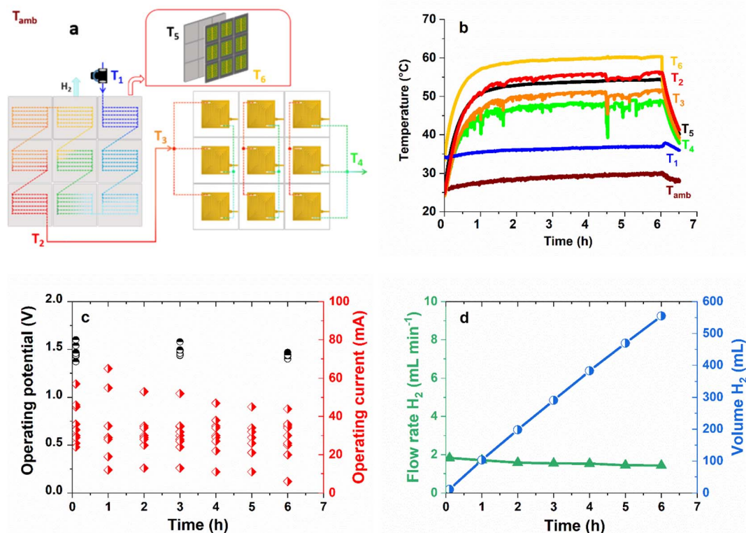
Fig. 4 IPEC module thermal integration and performance (68.4 cm 2 active area). (a) Detailed scheme of the water circuit in the IPEC module and (b) recorded temperatures. T_{\text{amb}} : ambient temperature. T_1 (blue): water inlet in the heat exchanger. T_2 (red): water outlet from the heat exchanger. T_3 (red): water inlet in the anodic compartment. T_4 (green): water outlet from the anodic compartment. T_5 (black): temperature of the cathodic plate. T_6 (yellow): temperature of the tandem solar cell. (c) Operating points ( V_{\text{op}} and I_{\text{op}} ) of the nine IPEC cells in the IPEC module before and during constant 1 sun illumination. (d) Calculated H 2 volume and flow rate produced by the IPEC module.
