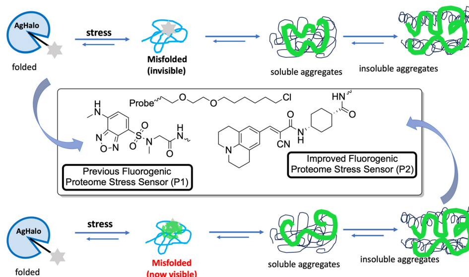
Fig. 4 Fluorogenic probes for the AgHalo sensor for understanding protein aggregation.
