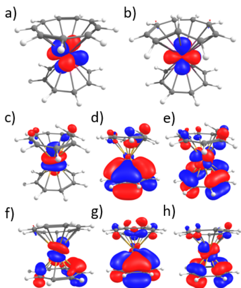
Fig. 9 Selected molecular orbitals (a) \alpha MO-HOMO-2 of 2-Ce- cis (SOMO). (b) \alpha MO-HOMO-2 2-Ce- trans (SOMO) (c) \alpha MO-HOMO-4 of 2-Sm- trans (d) \alpha MO-HOMO of 2-Sm- trans (e) \alpha MO-LUMO of 2-Sm- trans (f) \alpha MO-HOMO-8 of 2-Sm- cis (d) \alpha MO-HOMO of 2-Sm- cis (e) \alpha MO-LUMO of 2-Sm- cis .
