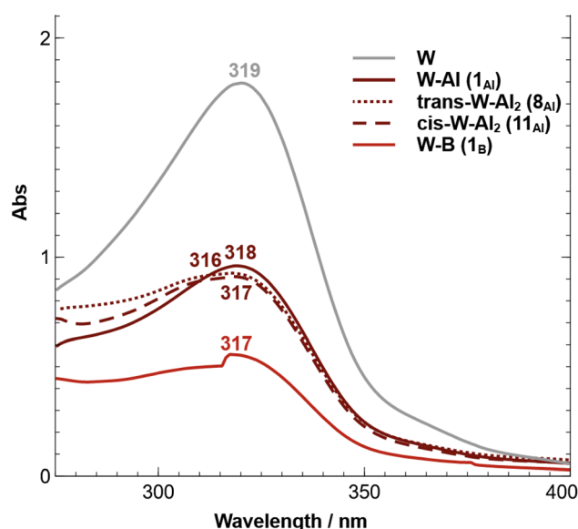
Fig. 9 Absorption spectra of trans - [W(depe)_2(N_2)_2] (W, grey line), trans - [W(depe)_2(N_2)(\mu\text{-N}_2\text{-Al}(C_6F_5)_3)] (W-Al, crimson line), trans - [W(depe)_2\{\mu\text{-N}_2\text{-Al}(C_6F_5)_3\}_2] ( trans -W-Al 2 , dotted crimson line), cis - [W(depe)_2\{\mu\text{-N}_2\text{-Al}(C_6F_5)_3\}_2] ( cis -W-Al 2 , dashed crimson line), and trans - [W(depe)_2(N_2)(\mu\text{-N}_2\text{-B}(C_6F_5)_3)] (W-B, red line). The concentration of each sample is about 30 \mu\text{M} .
