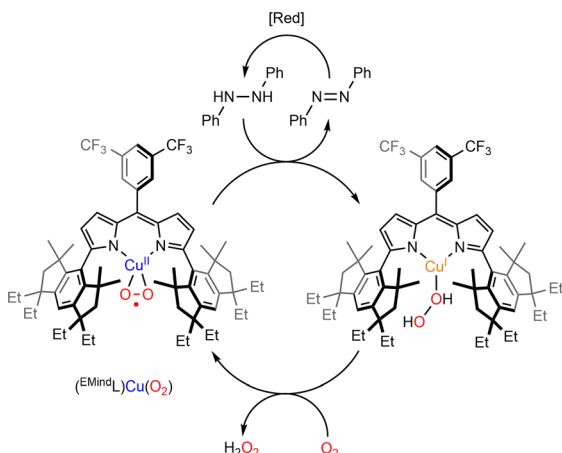
Scheme 7 Reaction of [(^{E_{Mind}}L)Cu^{II}(O_2)] with 1,2-diphenylhydrazine to produce azoarene and [(^{E_{Mind}}L)Cu^I(H_2O_2)] . Adapted from ref. 83.
