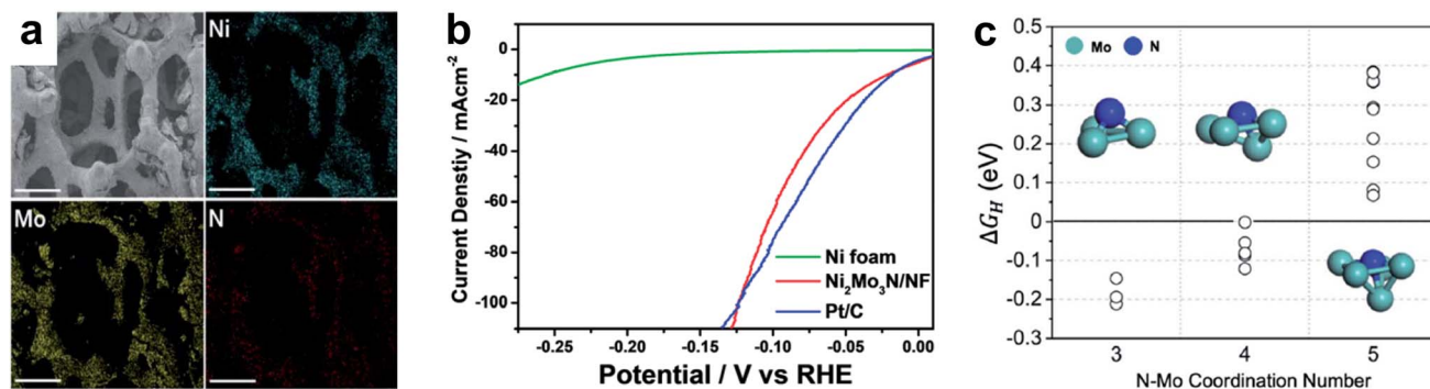
Fig. 9 (a) SEM-EDS of \text{Ni}_2\text{Mo}_3\text{N}/\text{NF} with scale bar of 300 \mu\text{m} . (b) LSV curves of Ni foam, \text{Ni}_2\text{Mo}_3\text{N}/\text{NF} , and \text{Pt}/\text{C} in 1.0 M KOH electrolyte. (c) The Gibbs free energy of adsorbed hydrogen ( \Delta G_{\text{H}} ) on different nitrogen adsorption sites with varying coordination number for N–Mo bonding. Reprinted from ref. 141 with permission from the Royal Society of Chemistry, Copyright 2021.
