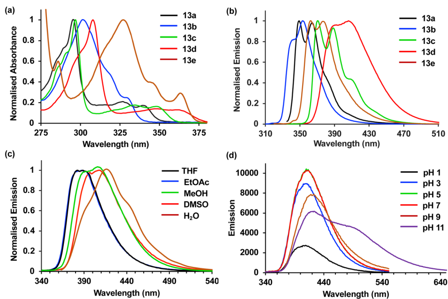
Fig. 3 (a) Absorption spectra of amino acids 13a–13e ( 5 \mu\text{M} ) in methanol. (b) Normalised emission spectra of amino acids 13a–13e ( 5 \mu\text{M} ) in methanol. (c) Normalised emission spectra of 13d ( 5 \mu\text{M} ) in various solvents. (d) Emission spectra of 13d ( 5 \mu\text{M} ) at various pH.
