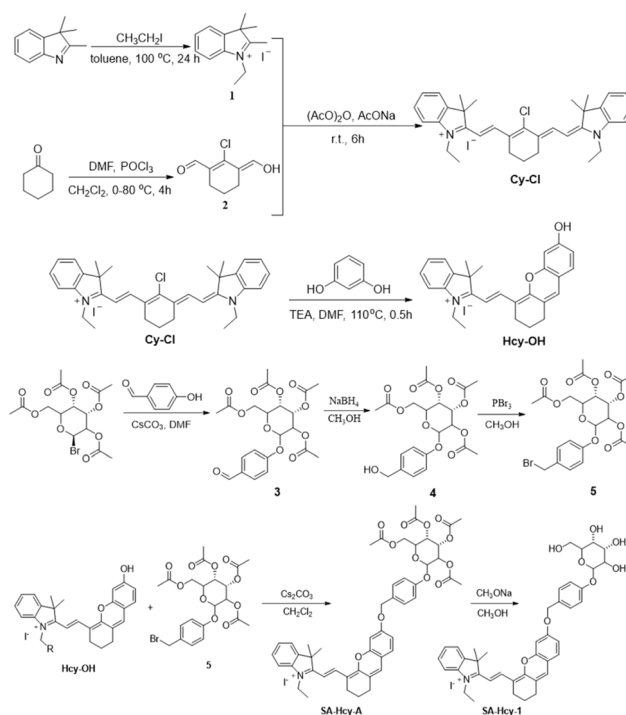
Scheme 2 Synthesis route of probe SA-HCy-1.
