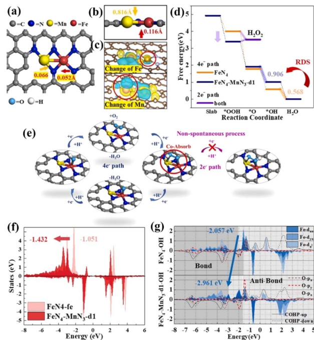
Fig. 17 (a) \text{FeN}_4\text{-MnN}_3\text{-d1} structure (d1 referring to the number of defect being 1). (b) Side view of the \text{FeN}_4\text{-MnN}_3 structure. (c) Charge density difference diagrams of \text{FeN}_4\text{-MnN}_3\text{-d1} . (d) Oxygen-free energy diagrams of \text{FeN}_4 and \text{FeN}_4\text{-MnN}_3\text{-d1} . (e) Illustrations of the ORR process on the \text{FeN}_4\text{-MnN}_3\text{-d1} structure. (f) The d-band changes of Fe in \text{FeN}_4 and \text{FeN}_4\text{-MnN}_3\text{-d1} . (g) PDOS of Fe in the d_{xz} , d_{yz} and d_{z^2} orbitals and the bonding and anti-bonding state information obtained by COHP. Reproduced with permission. 167 Copyright 2020, Elsevier B.V.
