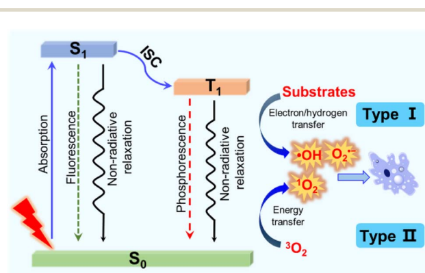
Fig. 1 The photosensitization process and photochemical reaction mechanisms of type I and type II PDT.
