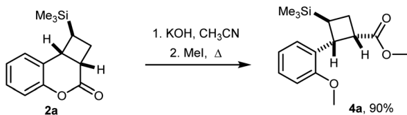
Scheme 3 One-step synthesis of D-A cyclobutane 4a from chromanone 2a .
