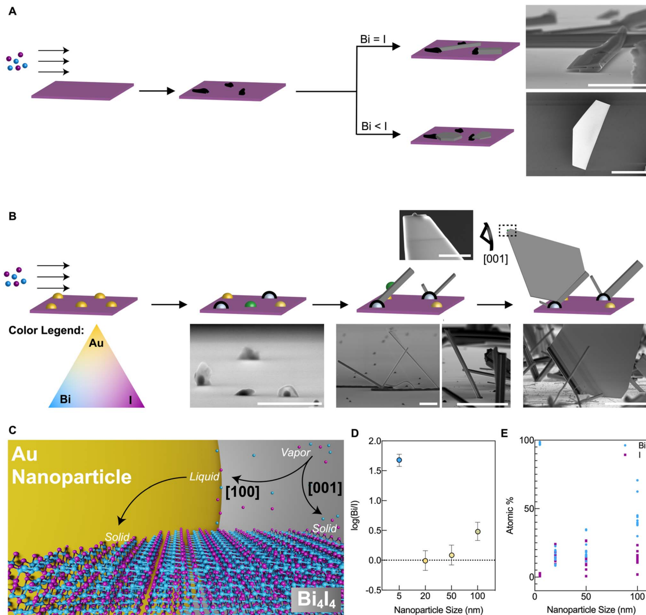
Fig. 4 Growth pathways involved in the crystallization of Bi 4 I 4 nanowires and quasi-2D nanosheets. (A) Schematic of the proposed CVD growth reaction pathway of Bi x I y nanocrystals in the absence of Au NPs. Black regions represent Bi x I y nucleation spots and gray particles represent the growing nanocrystals. SEM images of Bi 4 I 4 (Bi = I; Scale bar, 5 μm) and BiI 3 (Bi < I; scale bar, 50 μm) nanocrystals are included beside the corresponding schematic figure. (B) Schematic of the proposed CVD growth pathway of Bi 4 I 4 nanocrystals with Au NPs present on the growth substrate. A Bi/I/Au color legend for the depicted nanoparticles is added for better visualization. Green nanoparticles highlight Au NPs that are picked up by growing nanowires. SEM images of nanostructures corresponding to each step are shown below the schematic. Scale bars (from left to right): 500 nm, 1 μm, 10 μm, and 10 μm. A high-magnification SEM image of the tip of a flag-like quasi-2D nanosheet is included for reference. Scale bar, 2 μm. (C) Graphical representation of the dashed boxed region in the quasi-2D nanosheet in (B), depicting the VLS growth along the [100] vdW direction and VS growth along the [001] vdW direction. (D) and (E) Dependence of Bi and I dissolution on the diameters of Au NPs presented as Bi-to-I ratios plotted in a logarithm scale (D) and atomic percentages of Bi and I (E). Values shown in (D) and (E) were derived from EDS compositions of on-substrate nanoparticles post-reaction ( n = 10 particles per Au NP diameter).
