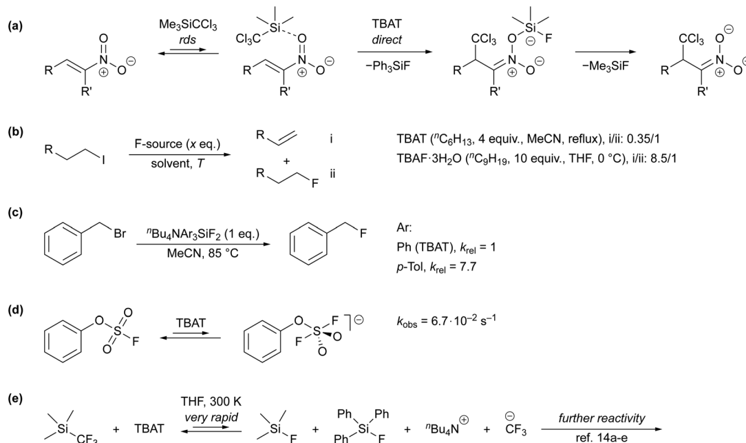
Scheme 1 (a) Mechanistic proposal in a study on the addition of \text{TMS-Cl}_3 to nitroalkenes, 10 (b) ratios of \beta -elimination-to-substitution products in reactions of 1-iodoalkanes with TBAT and \text{TBAF} \cdot 3\text{H}_2\text{O} , 11 (c) relative rate constants of fluorination of benzyl bromide using ^n\text{Bu}_4\text{NAr}_3\text{SiF}_2 , where Ar = Ph or p -Tol, 12 (d) rapid fluoride exchange between TBAT and phenyl fluorosulfate studied via time-dependent saturation transfer NMR spectroscopy, 13 (e) prior mechanistic work on TBAT-initiated reactivity of \text{TMS-CF}_3 , where the fluoride transfer from TBAT is very rapid with respect to NMR spectroscopy. In the presence of excess \text{TMS-CF}_3 , the \text{CF}_3^- anion(oid) is transient, undergoing rapidly-reversible exergonic equilibrium with [\text{TMS}(\text{CF}_3)_2]^- . 14
