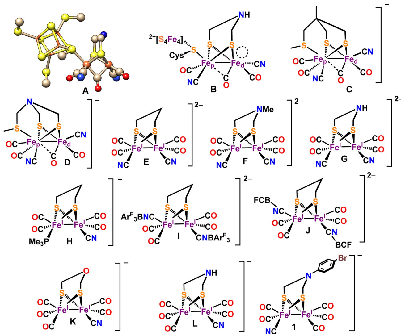
Scheme 1 (A) X-ray crystal structure of the "H-cluster" in the \text{H}_{\text{ox}} state in [\text{Fe}-\text{Fe}]\text{-H}_2 ase (PDB ID: 3C8Y 62 ). (B) Chem Draw representation of the active site of [\text{Fe}-\text{Fe}]\text{-H}_2 ase. The vacant site at the distal iron atom is indicated by a circular ring. Reported [\text{Fe}-\text{Fe}] \text{H}_2 ase synthetic mimics bearing -\text{CN} ligands in \text{H}_{\text{rest}} (C-L). New synthetic mimic of [\text{Fe}-\text{Fe}] \text{H}_2 ase [\text{BrC}_6\text{H}_4\text{N}(\text{CH}_2\text{S})_2\text{Fe}_2(\text{CO})_5\text{CN}]^- (1).
