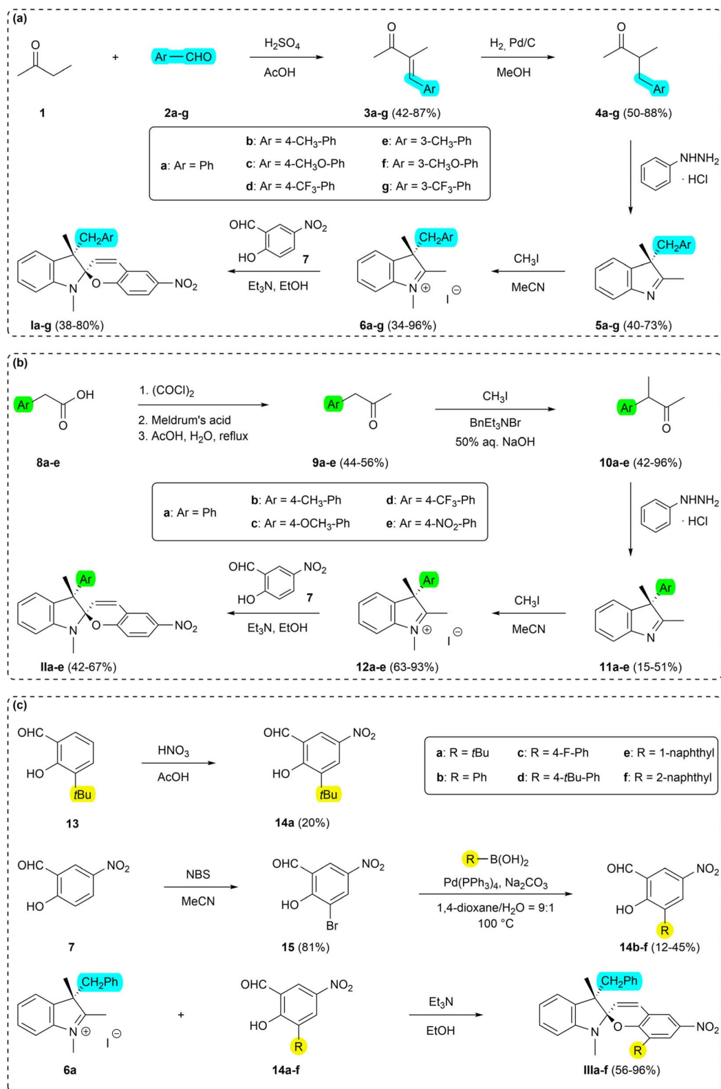
Scheme 2 Synthesis of the target spiroopyrans: (a) 1a-g (Series I), (b) 11a-e (Series II), (c) 11a-f (Series III).
