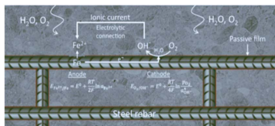
Fig. 2 Corrosion process a schematic view of oxidation and anodic, cathodic reaction. 12
