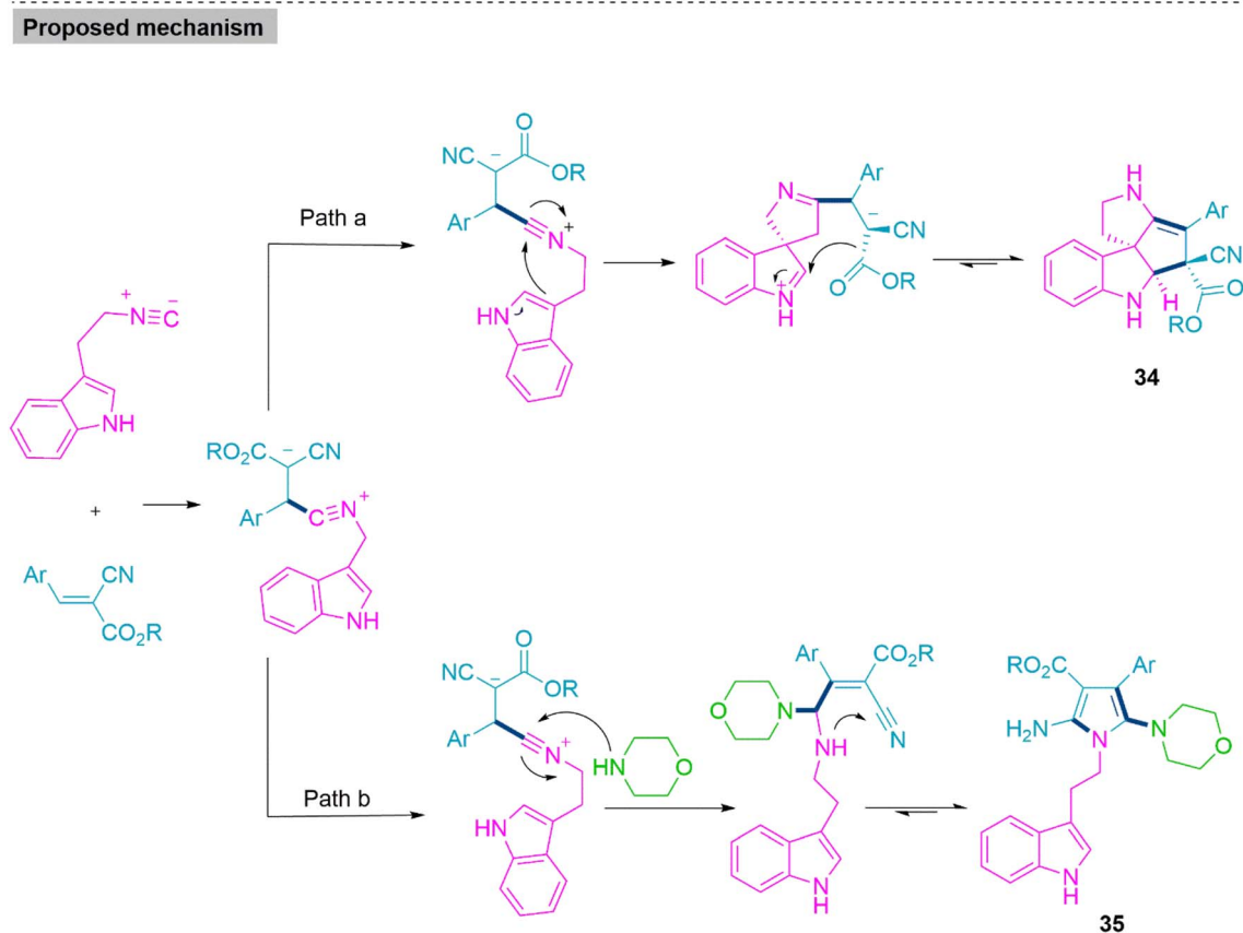
Scheme 19 Synthesis of spiroindoline ( 34 ) and functionalized pyrrole derivatives ( 35 ).
