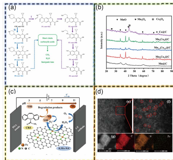
Fig. 8 (a) Proposed pathways for degradation of CIP. (b) XRD patterns of Mn_xCo_{3-x}@C (this figure has been reproduced with permission from Huang S. et al. 77 from Elsevier, copyright 2022). (c) Schematic diagram of possible CBZ degradation mechanism by 0.3Fe-N/C/hetero-EF. (d) HAADF-STEM and corresponding element maps of 0.3Fe-N/C (this figure has been reproduced with permission from Guo J. et al. 78 from Elsevier, copyright 2022).
