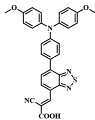
(28) MPA-BT-CA (PCE=21.24%)
