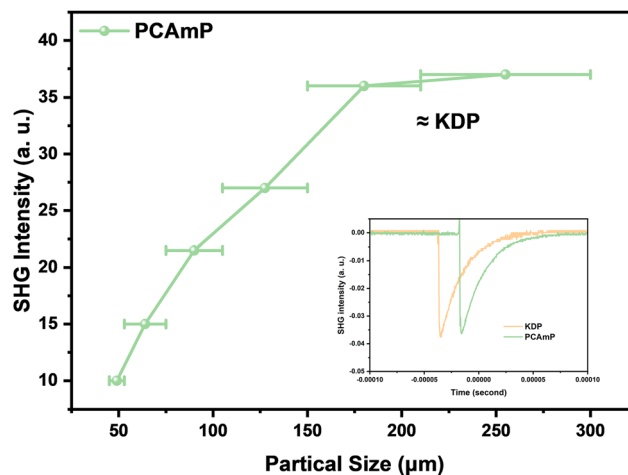
Fig. 5 Phase-matching curve of I with 1064 nm laser radiation (insert is oscilloscope traces of the SHG signals for powders of I and KDP (150–210 µm) with 1064 nm laser radiation).
