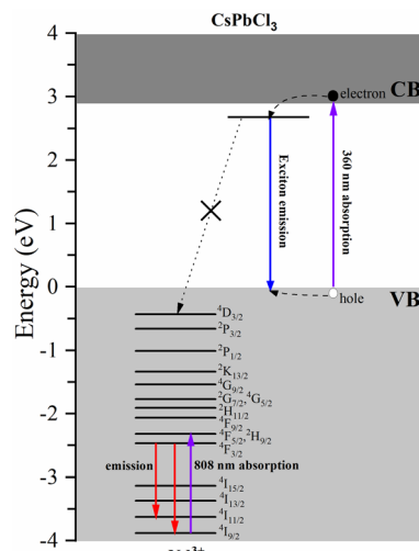
Fig. 10 Electronic energy level scheme determined for the CsPbCl 3 :Nd 3+ perovskite powder.
