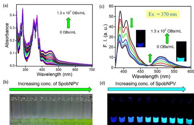
Fig. 2 (a) UV-vis titration of compound 1 ( 10\ \mu\text{M} ) with SpobNPV ( 0 – 1.3 \times 10^7 OBs \text{mL}^{-1} ) in water. (b) Change in color of the aqueous solution of 1 ( 10\ \mu\text{M} ) upon gradually adding SpobNPV in water. (c) Fluorescence spectral titration of compound 1 ( 10\ \mu\text{M} , \lambda_{\text{ex}} = 370\ \text{nm} ) with SpobNPV ( 0 – 1.3 \times 10^7 OBs \text{mL}^{-1} ) in water. (d) Change in the color of the aqueous solution of 1 ( 10\ \mu\text{M} ) upon gradual addition of a suspension of SpobNPV in water under a UV lamp ( >365\ \text{nm} ).
